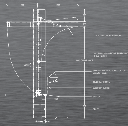
Section View - through opening at window
